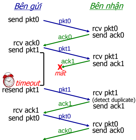
(c) Mất ACK
